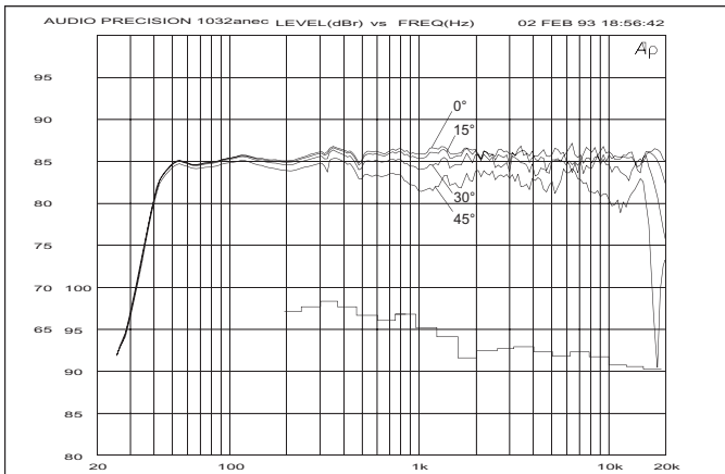
Figure 4. The upper curve group shows the horizontal directivity characteristics of the 1032A in vertical configuration measured at 1 m. The lower curve is a 1/3 octave band power response, measured in an IEC approved reverberation chamber.
