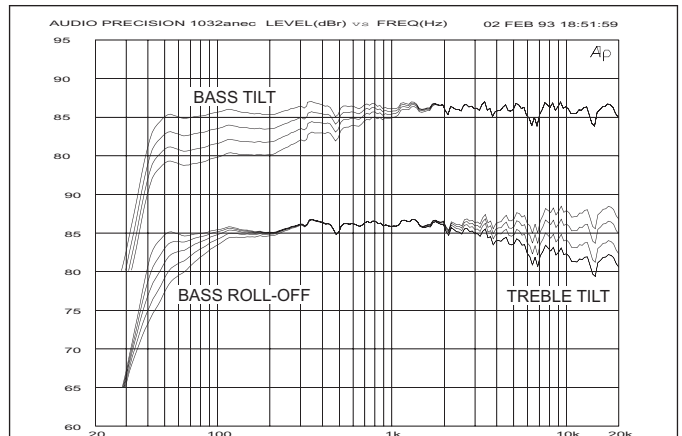
Figure 5. The upper curve group shows the effect of the bass tilt control on the free field response. The lower curves show the effect of the treble tilt and bass roll-off controls.
