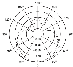
TYPICAL POLAR PATTERNS
