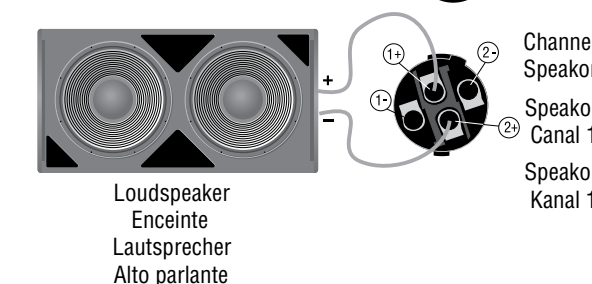
Figure 2.13 Alternate Bridge-Mono Wiring: Loudspeaker Wired to Amplifier's Top Speakon® Connector
