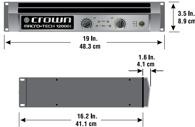
Figure 2.1 Dimensions
