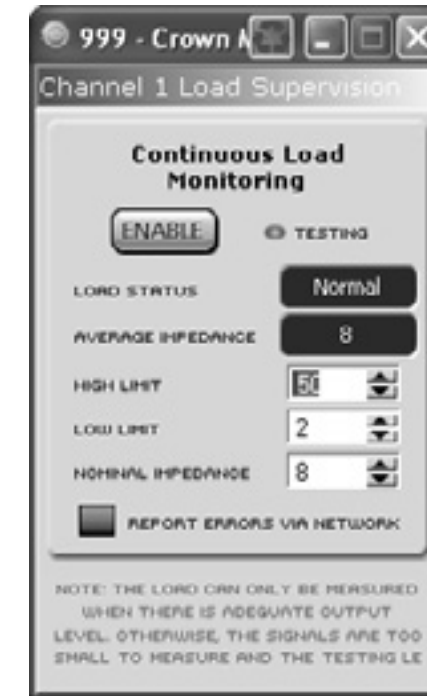
Figure 4.6 MA-i Load Monitoring Panel
