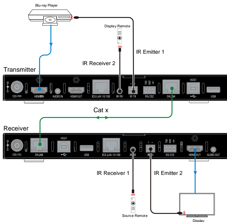
Fig 2: IR Pass-Through
